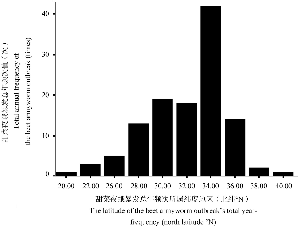
图 2 中国甜菜夜蛾暴发频次的地理纬度分布比较图 Fig. 2 The chart of latitude distribution in outbreak frequency of the beet armyworm in China
