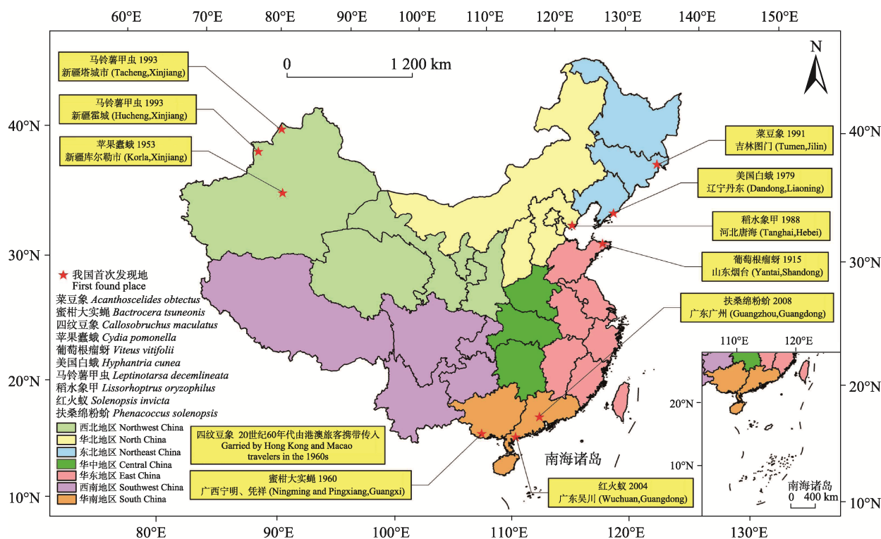
Fig. 1 First found places and times of national quarantine insects of agricultural plants in China
