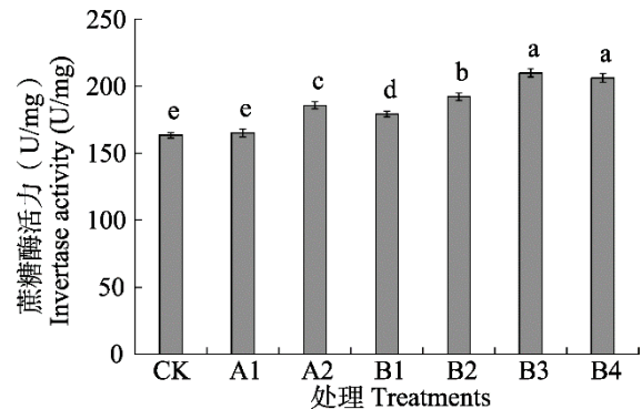
图4 蚜害棉花对棉蚜蔗糖酶活性的影响 Fig. 4 Effects of aphid infestation on invertase activity of Aphis gossypii
