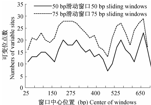
图 2 翁蛭螂属COI 序列可变量点数的滑动窗口分析 Fig.2 Sliding windows analysis( variable sites,S) among COI sequences of Onthophagus species
