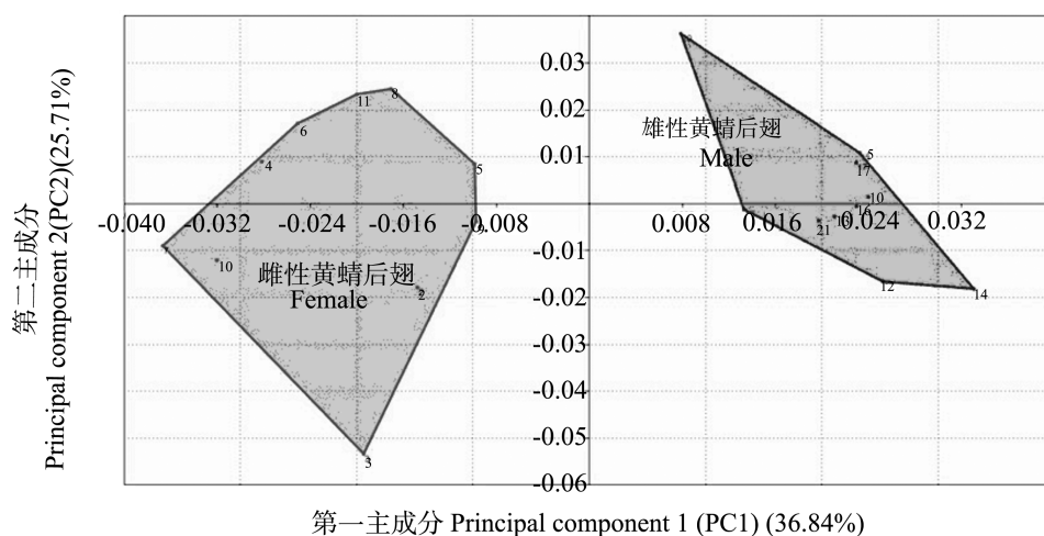
图 4 雌性黄蜻和雄性黄蜻后翅第一主成分 (PC1) 和第二主成分 (PC2) 散点图 Fig. 4 The first principal component (PC1) and the second principal component (PC2) scatter plots of the hindwing between female and male of Pantala flavescens
