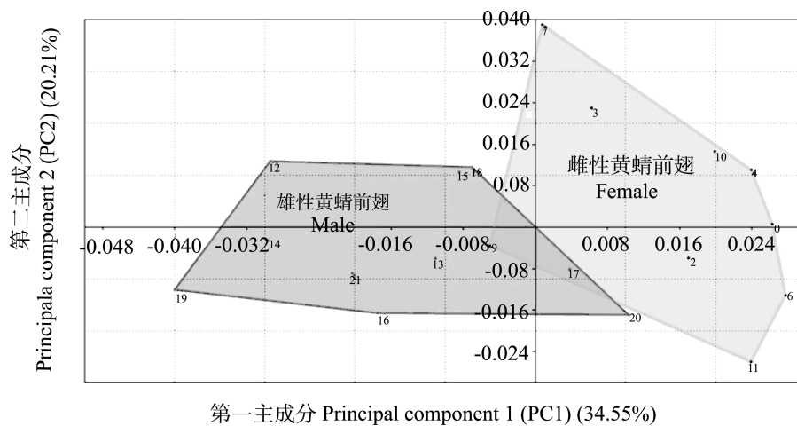
图 3 雌性黄蜻和雄性黄蜻前翅第一主成分 (PC1) 和第二主成分 (PC2) 散点图 Fig. 3 The first principal component (PC1) and the second principal component (PC2) scatter plots of the forewing between female and male of Pantala flavescens
