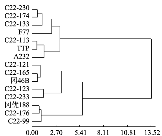
图 4 供试材料对三化螟产卵抗性聚类 Fig. 4 Cluster of the materials resistance to oviposition of Tryporyza incertulas
