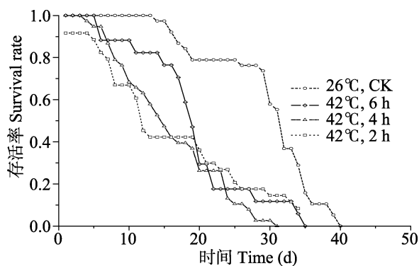
图 2 42℃高温处理下双尾新小绥螨雌成螨的存活率 Fig. 2 Survival rates of female adults of Neoseiulus bicaudus after exposure to 42℃
