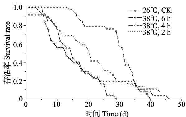
图 1 38℃高温处理下双尾新小绥螨雌成螨的存活率 Fig. 1 Survival rates of female adults of Neoseiulus bicaudus after exposure to 38℃
