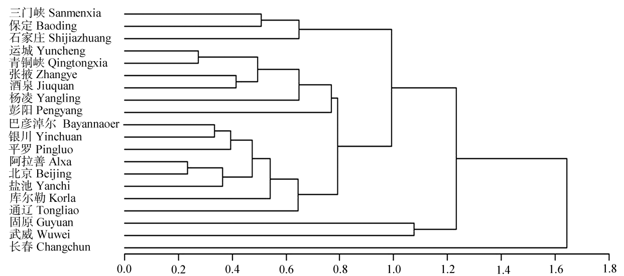
图 3 基于表型性状的聚类图 Fig. 3 Dendrogram analysis based on phenotypic traits
