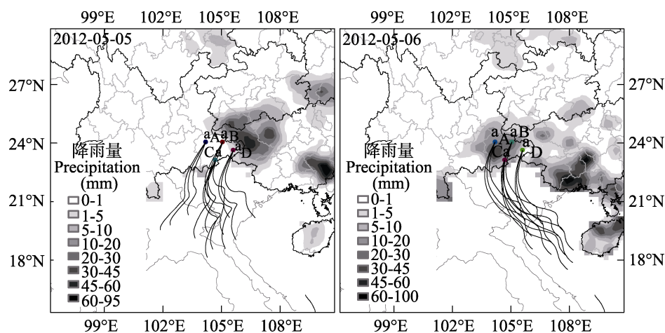
图 10 2012 年 5 月 5—6 日滇东南白背飞虱迁飞路径回推轨迹和累计降雨量 Fig. 10 The backward trajectories and the accumulated precipitation of Sogatella furcifera in southeast Yunnan in the past 24 hours during 5 to 6 May, 2012
