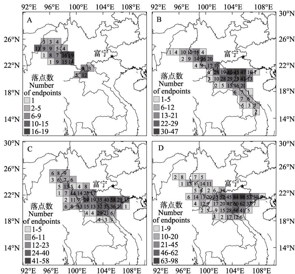
图 2 2008—2012 年 4—5 月富宁白背飞虱虫源地分布 Fig. 2 The distribution of source area of immigrating WBPH in Funing in April and May during 2008 to 2012 A. 4 月 ; B. 5 月上旬 ; C. 5 月中旬 ; D. 5 月下旬。 A. April; B. The first ten days of May; C. The second ten days of May; D. The last ten days of May.
