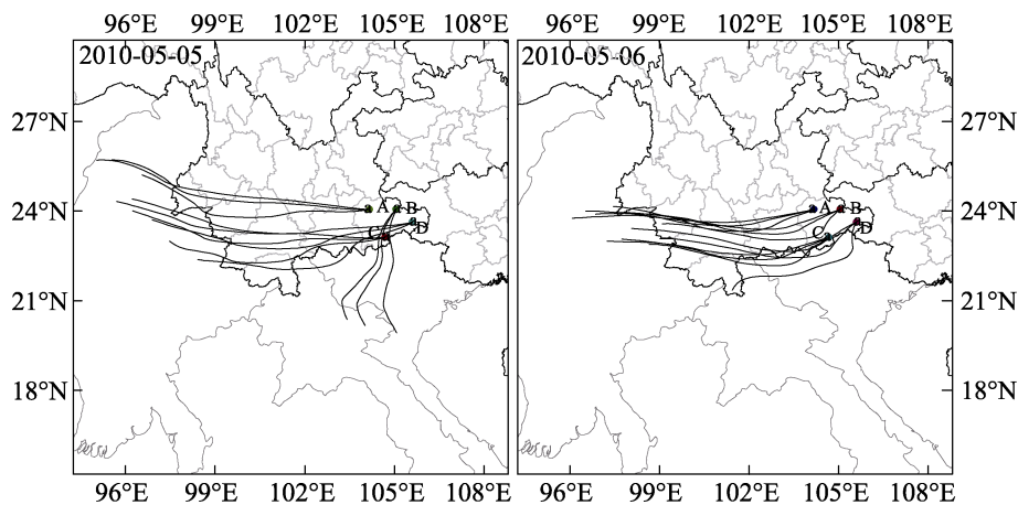
图 13 2010 年 5 月 5 日和 6 日滇东南白背飞虱迁飞路径轨迹回推 Fig. 13 The backward trajectories of Sogatella furcifera in southeast Yunnan during 5 to 6 on May, 2010
