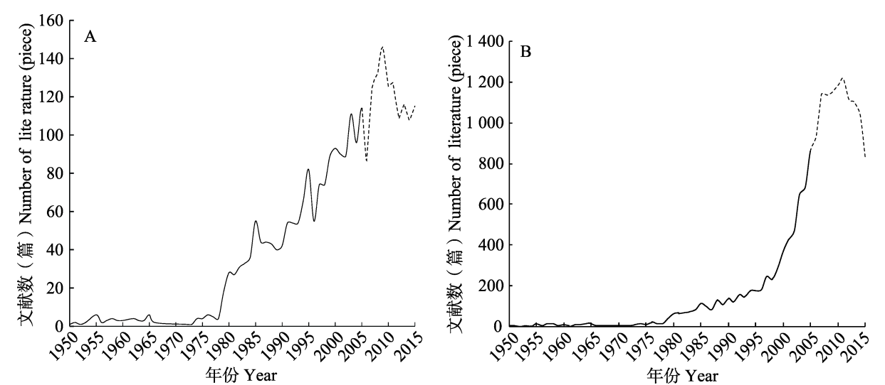
图 4 基于主题 (A) 和全文 (B) 检索的同翅目使用情况的时间趋势 Fig. 4 Time-series trends of the usage of Homoptera in Chinese scientific papers based on subject (A) and full text (B) searches
