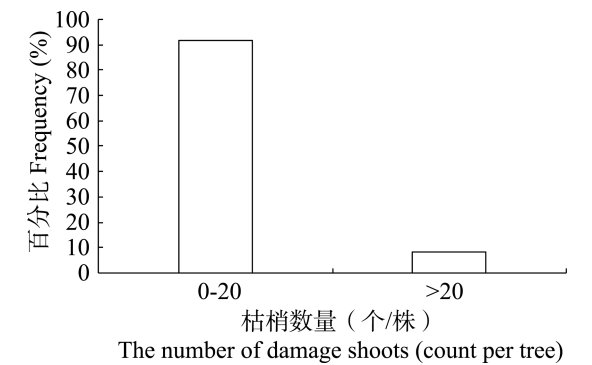
图 2 轻度受害林分受害梢密度分布 Fig. 2 Histogram of density for damage shoots in lightly-infested forest
