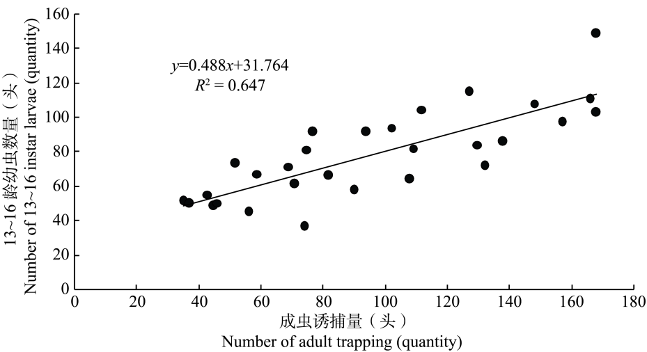
图 2 幼虫数量与诱捕量散点图 Fig. 2 Scatter plot of the number of larvae and trapping
