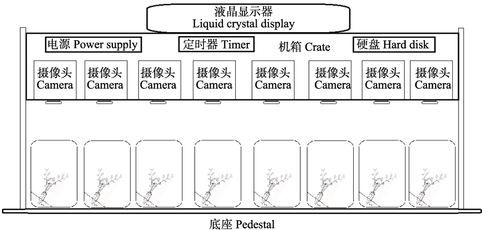
图 1 行为观测仪观测方法简图 Fig. 1 The sketch of observation method under the insect behavioral observer
