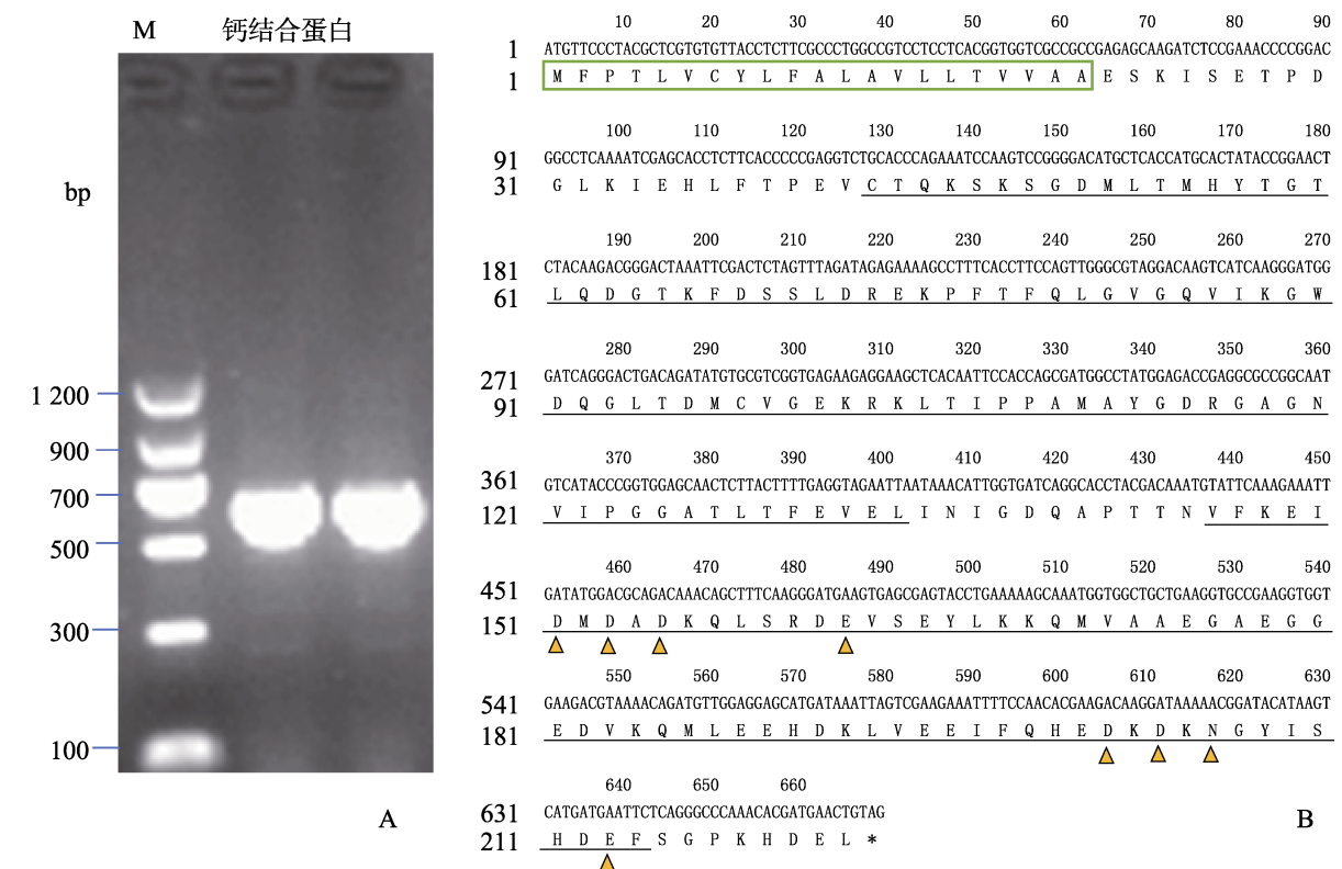
图 1 钙结合蛋白序列分析 Fig. 1 Analysis of calcium-binding protein sequence A. 钙结合蛋白全长克隆；B. 烟粉虱钙结合蛋白核酸序列及其编码的氨基酸序列。M：DNA 分子质量标准；钙结合蛋白：两个重复的 PCR 产物图。方框内为预测的信号肽，黑色单下划线为两个保守结构域，三角标记为钙结合位点。 A. Amplification of calcium-binding protein; B. Nucleotide and deduced amino acid sequences of calcium-binding protein . M: DNA molecular weight marker; Calcium-binding protein: Two PCR product. Within the box is the predicted signal peptide, black underlined for two conserved domains, and triangle labeled for Ca 2+ binding sites.
