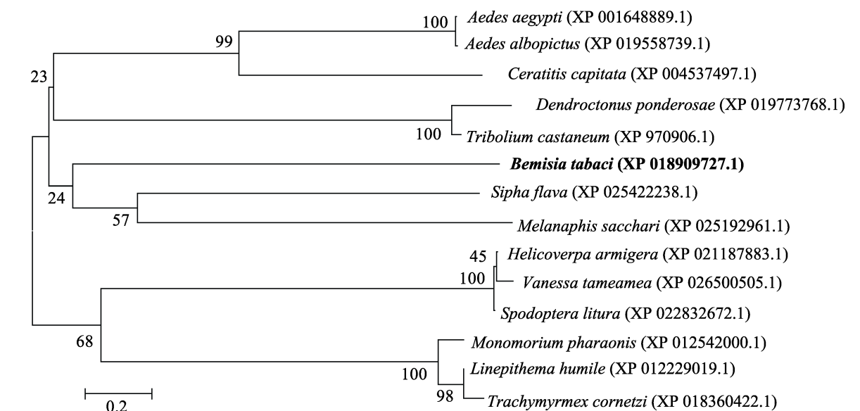
图 2 烟粉虱钙结合蛋白与其他昆虫的系统进化分析 Fig. 2 Phylogenetic relationships of calcium-binding protein sequences from Bemisia tabaci and other insects
