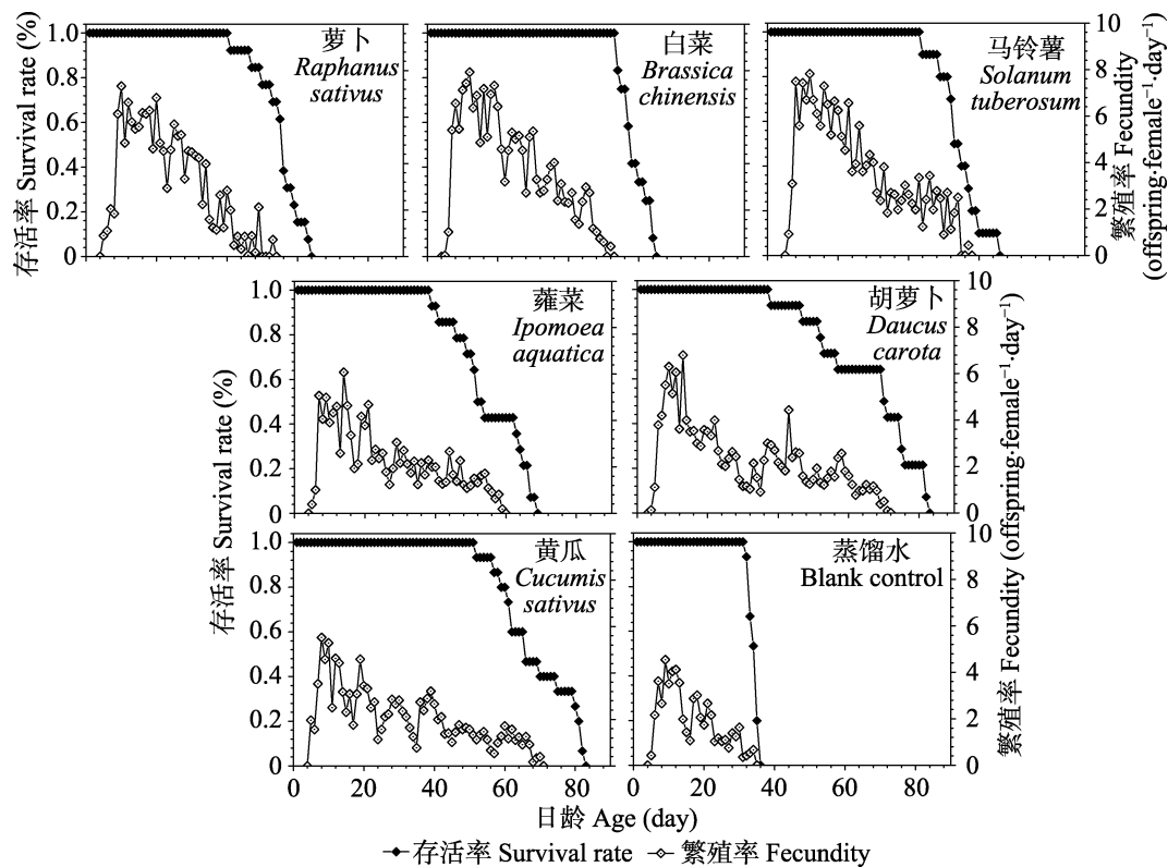
图 1 不同种类蔬菜条件下黄粉虫成虫的存活率和特定年龄繁殖率 Fig. 1 Proportion of population surviving and age-specific fecundity of Tenebrio molitor fed on different kinds of vegetable at (25±1)°C, RH 70%±5% and dark conditions
