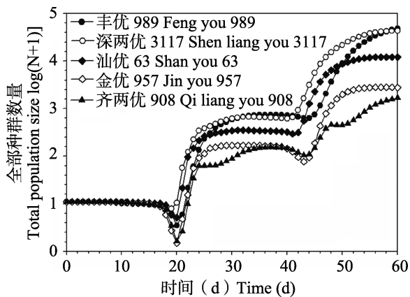
图 2 5 种水稻 (“深两优 3117”、“金优 957”、“齐两优 908”、“丰优 989”、“汕优 63”) 对褐飞虱的种群数量模拟 Fig. 2 Population number simulation of Nilaparvata lugens feeding on five rice varieties (“Shen liang you 3117”, “Jin you 957”, “Qi liang you 908”, “Feng you 989” and “Shan you 63”)
