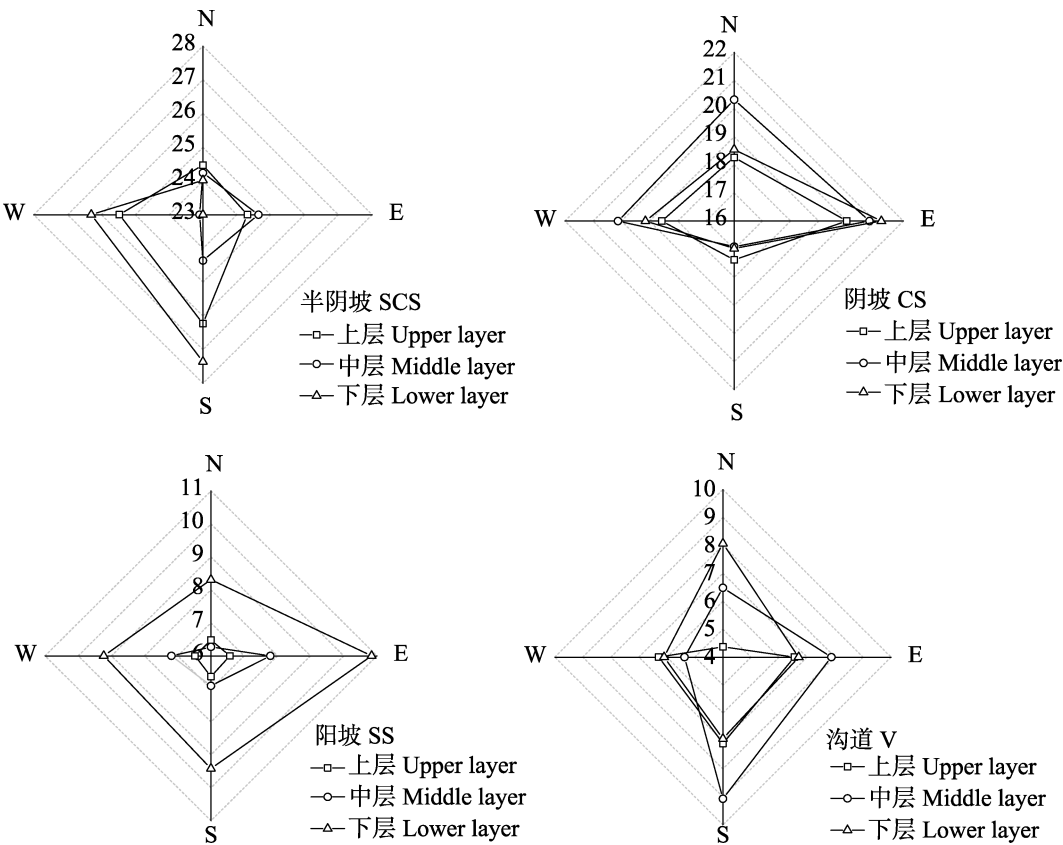
图 3 榆跳象幼虫不同坡向、方向及冠层幼虫密度雷达图 Fig. 3 Radar chart of density for the larvae in different aspects, direction and canopy
