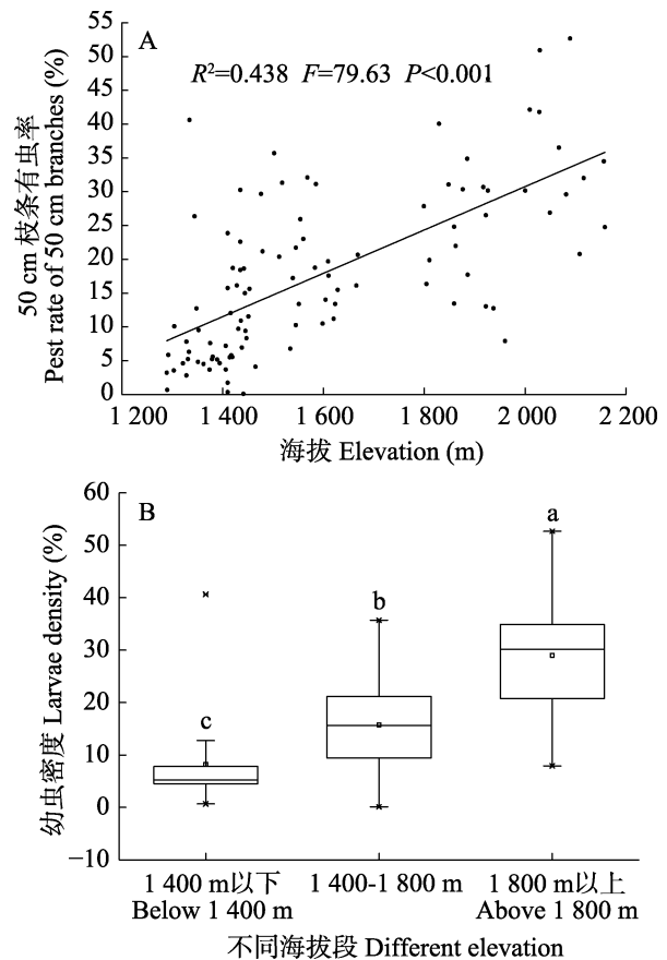
图 5 榆跳象幼虫密度与灰榆林海拔的关系 Fig. 5 Larvae density of grey elm trees in different elevation
