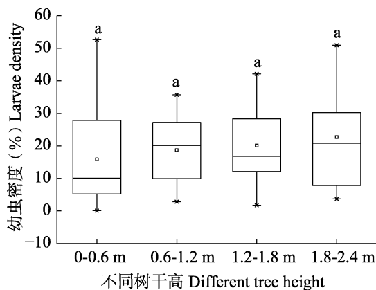
图 4 不同树干高榆跳象幼虫密度 Fig. 4 Larvae density of grey elm trees in different tree height
