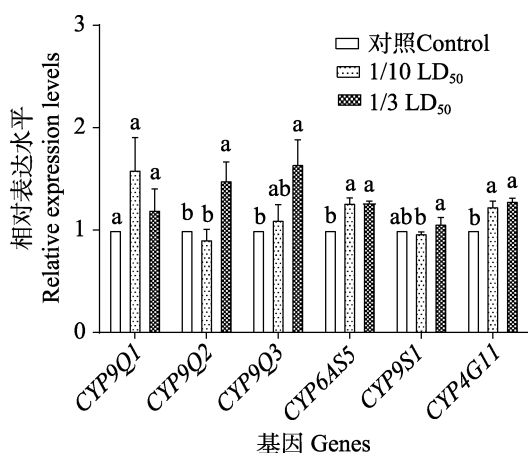
图 2 氟啉虫胺腈对蜜蜂 6 种解毒相关基因表达的影响 Fig. 2 Effects of sulfoxaflo on six detoxification related genes in honeybees ( Apis mellifera ligustica )
