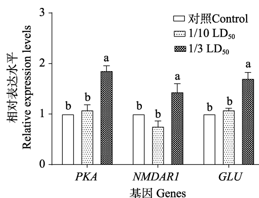
图 4 氟啉虫胺腈对蜜蜂 3 种记忆相关基因表达的影响 Fig. 4 Effects of sulfoxaflo on three memory related genes in honeybees ( Apis mellifera ligustica )
