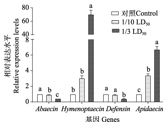
图 3 氟啉虫胺腈对蜜蜂 4 种免疫相关基因表达的影响 Fig. 3 Effects of sulfoxaflo on four immune related genes in honeybees ( Apis mellifera ligustica )
