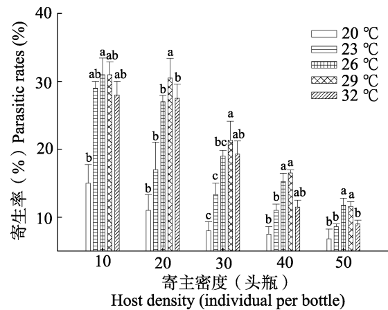
图 1 不同温度下淡足侧沟茧蜂对草地贪夜蛾的寄生情况 Fig. 1 Parasitic rates of Microplitis pallidipes on Spodoptera frugiperda larvae at different temperatures
