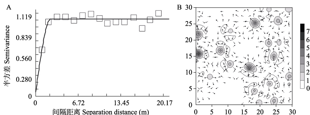
图 3 中度受害林内侵入孔数量的半变异函数图 (A) 和等值线与矢量叠加图 (B) Fig. 3 Semivariogram (A), overlay map of isoline and vector (B) of the number for entrance holes in moderate-infested forests
