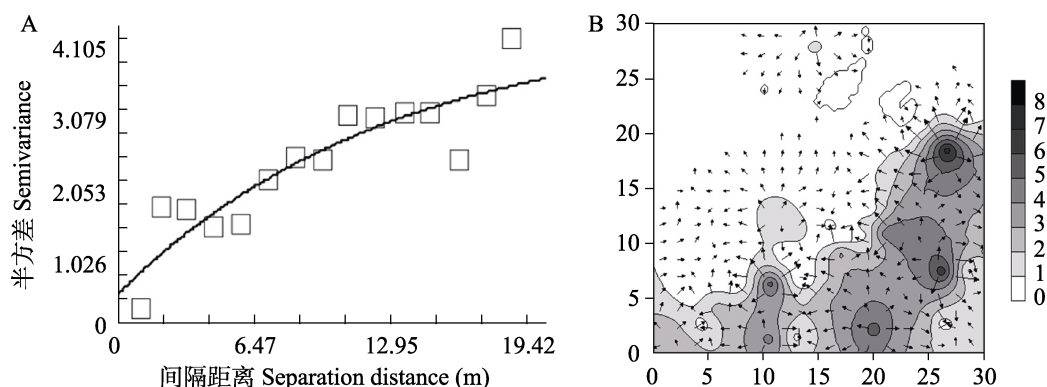
图 4 重度受害 (过火) 林内侵入孔数量的半变异函数图 (A) 和等值线与矢量叠加图 (B) Fig. 4 Semivariogram (A), overlay map of isoline and vector (B) of the number for entrance holes in severe-infested (post-fire) forests
