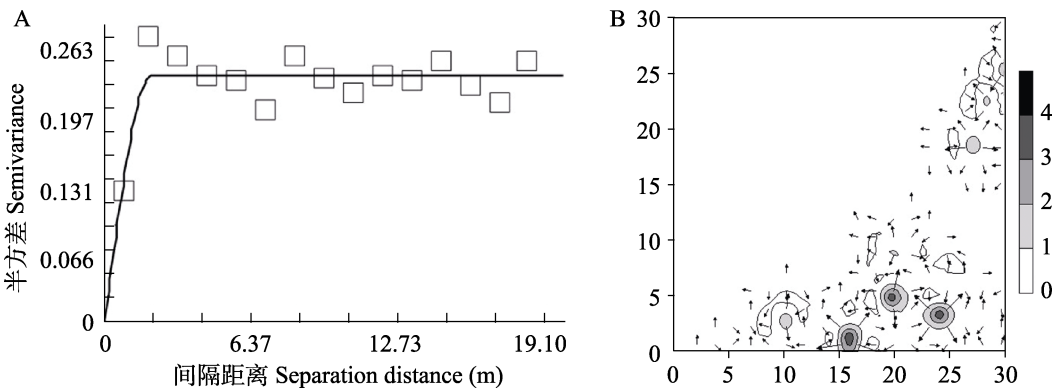
图 2 轻度受害林内侵入孔数量的半变异函数图（A）和等值线与矢量叠加图（B） Fig. 2 Semivariogram (A), overlay map of isoline and vector (B) of the number for entrance holes in lightly infested forests
