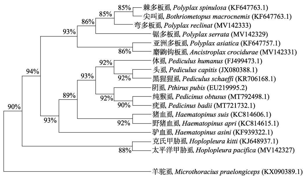
图 2 用 MP 法构建表种吸虱 trnL 1 (tag) 基因序列的进化关系 Fig. 2 Evolutionary relationship inferred from trnL 1 (tag) gene sequence of 17 species of sucking lice using MP methods
