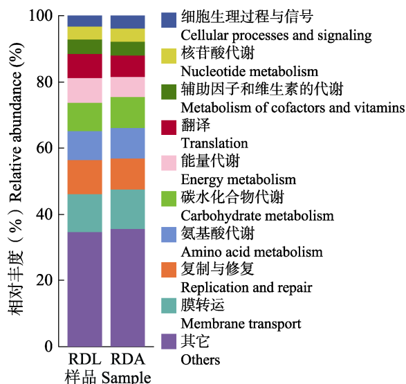
图 4 谷蠹幼虫和成虫体内细菌基因功能注释相对丰度柱形图 Fig. 4 Relative abundance and gene function annotation of the bacteria in larvae and adults of Rhizopertha dominica
