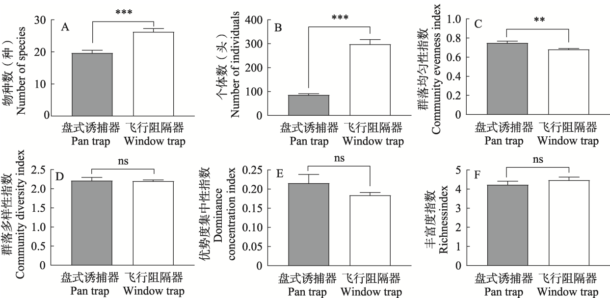
图 2 盘式诱捕器与飞行阻隔器的 \alpha 多样性性比较 Fig. 2 A comparison of \alpha diversity between pan trap and window trap
