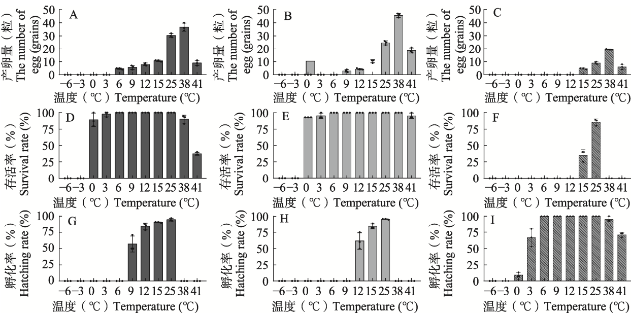
图 5 温度处理对不同季节采集的柑桔全爪螨的影响 Fig. 5 Various temperature treatments induced effects to Panonychus citri collected from different seasons
