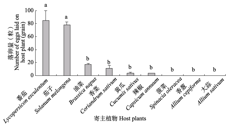
图1 5对番茄潜叶蛾雌雄成虫在不同寄主植物上的总产卵量 Fig. 1 The total number of eggs laid by 5 pairs of Tuta absoluta female and male adult on different host plants
