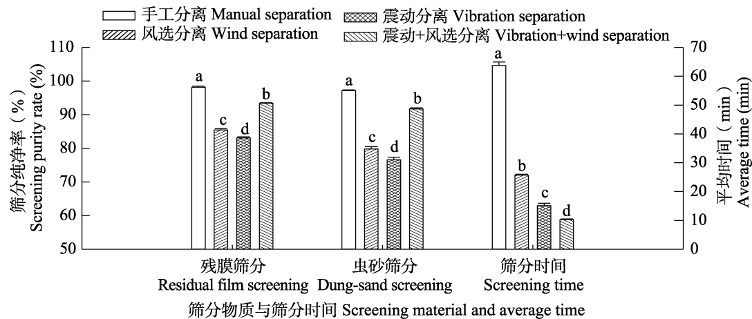
图 3 不同筛分方式对残膜、虫砂筛分效率的影响 Fig. 3 Effects of different screening methods on screening efficiency of residual film and dung-sand
