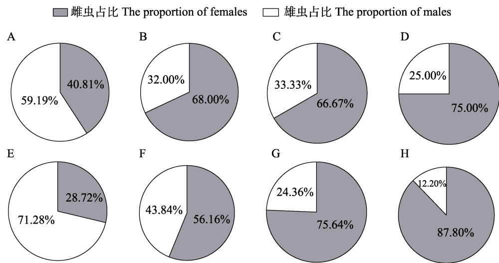
图 2 2023 和 2024 年玉米田双斑长跗萤叶甲雌雄成虫数量比 Fig. 2 Proportions of male to female Monolepta hieroglyphic adults in maize field in 2023 and 2024 A. 2023 年大喇叭口期雌雄成虫数量比; B. 2023 年抽雄吐丝期雌雄成虫数量比; C. 2023 年灌浆期雌雄成虫数量比; D. 2023 年乳熟期雌雄成虫数量比; E. 2024 年大喇叭口期雌雄成虫数量比; F. 2024 年抽雄吐丝期雌雄成虫数量比; G. 2024 年灌浆期雌雄成虫数量比; H. 2024 年乳熟期雌雄成虫数量比。 A. Proportions of male to female adults in the vegetative 12 stage in 2023; B. Proportions of male to female adults in the tasseling and silking stage in 2023; C. Proportions of male to female adults in the blister stage in 2023; D. Proportions of male to female adults in the milk stage in 2023; E. Proportions of male to female adults in the vegetative 12 stage in 2024; F. Proportions of male to female adults in the tasseling and silking stage in 2024; G. Proportions of male to female adults in the blister stage in 2024; H. Proportions of male to female adults in the milk stage in 2024.
