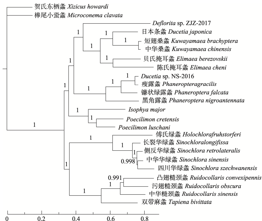
Fig. 4 Phylogenetic tree in Phaneropterinae
