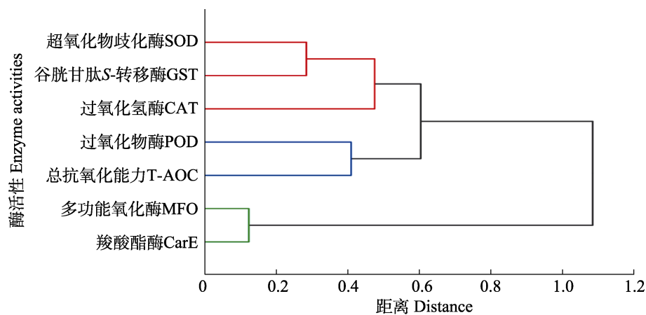
图 9 温度胁迫下酶活性聚类结果 Fig. 9 Clustering results of enzyme activities under ambient temperature stress
