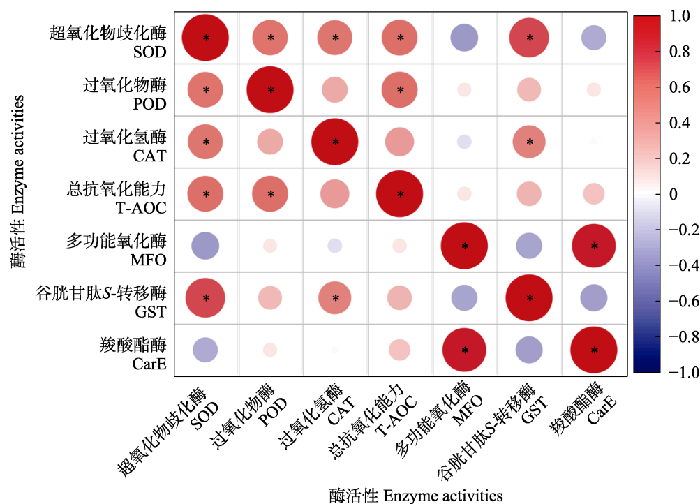
图 8 抗氧化酶与解毒酶活性的相关性结果 Fig. 8 Correlation results between antioxidant enzymes and detoxification enzyme activities *代表经 Pearson 法分析差异显著 ( P < 0.05 )。 * represents significant difference as determined by Pearson's correlation analysis ( P < 0.05 ).
