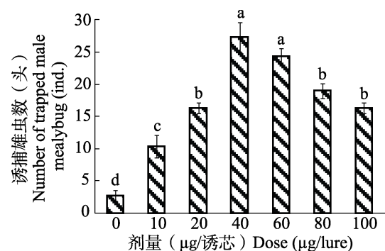
图 2 不同剂量扶桑绵粉蚧性信息素对雄虫引诱效果 Fig. 2 Trapping efficiency of different doses of the synthetic sex pheromone of Phenacoccus solenopsis
