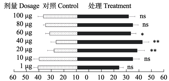
图 1 扶桑绵粉蚧雄虫对不同浓度性信息素趋向反应 Fig. 1 Response of Phenacoccus solenopsis adult males to different concentrations of sex pheromone
